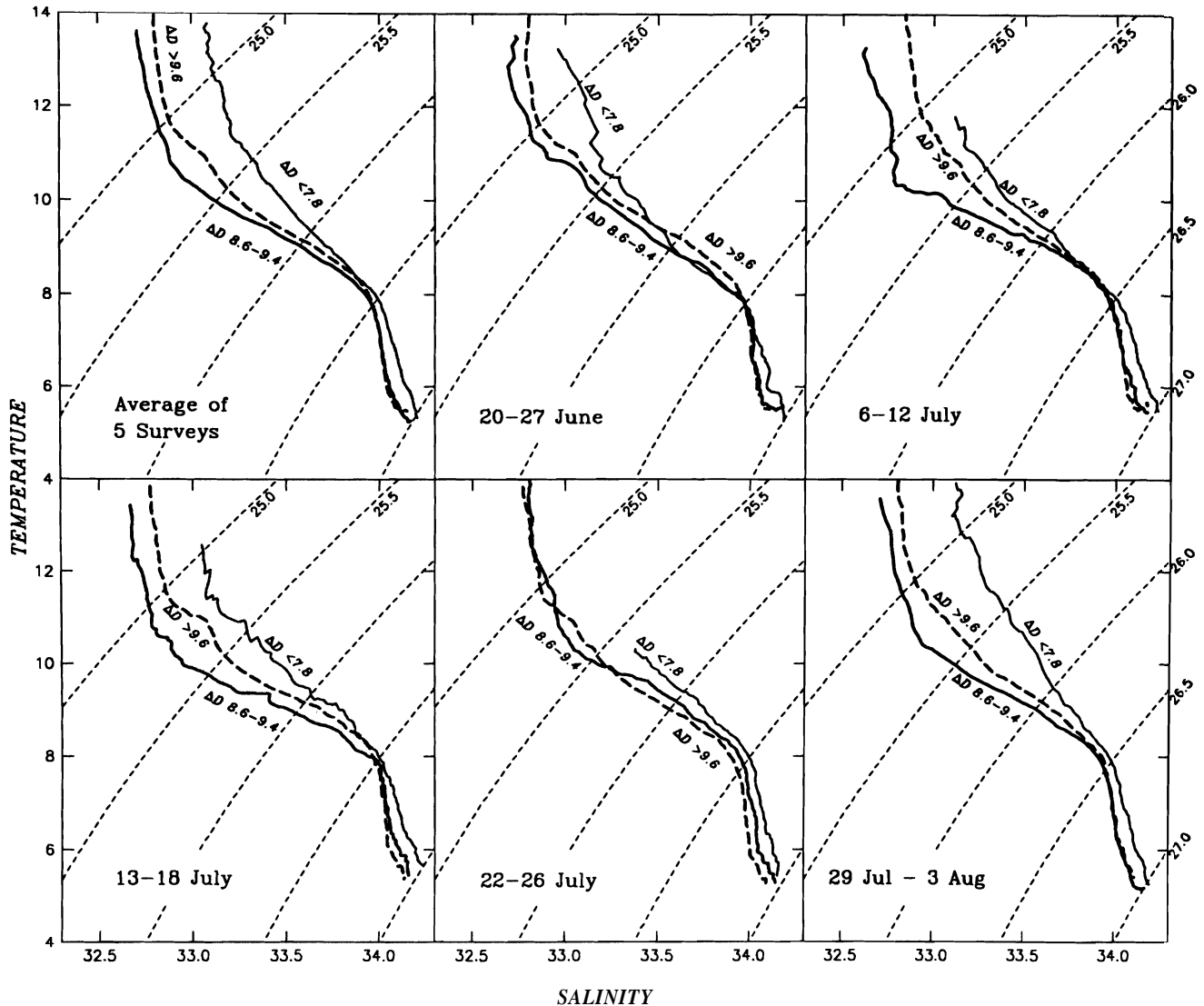
Fig. 16. Average T-S curves for the inshore, offshore, and jet core stations for each of the five surveys. Curves are shown only for the density range covered by at least four stations. (The top left panel repeats the average curves of Figure 15 for comparison).
