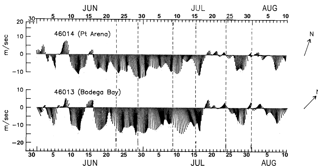
Fig. 2. Low-passed ( <0.6 cpd) vector time series of the wind measured at NDBC buoys near Point Arena (relative to 341^\circ\text{T} ) and Bodega Bay (relative to 316^\circ\text{T} ). Vertical lines indicate the mid-point of each survey.
