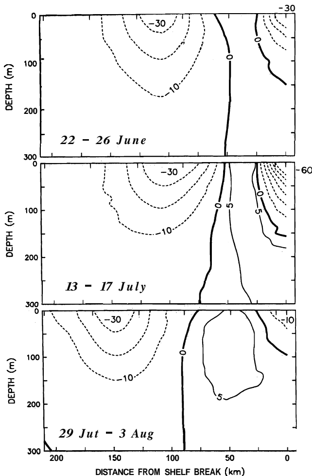
Fig. 9. Onshore-offshore sections of geostrophic velocity (relative to 500 dbar) along the line connecting F5 to B5, A8, and A9, at the beginning, middle, and end of the survey sequence.
