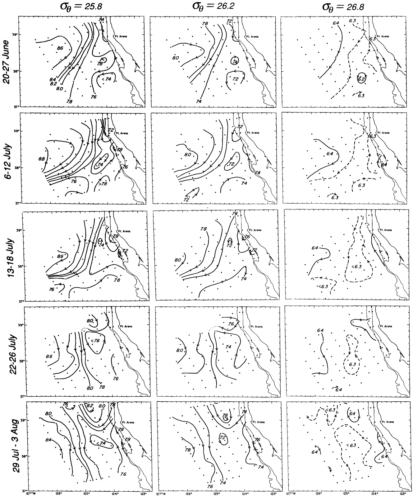
Fig. 19. Acceleration potential ( \text{m}^2 \text{s}^{-2} ) on the isopycnal surfaces on which \sigma_\theta is 25.8, 26.2, and 26.8, for the five complete surveys.
