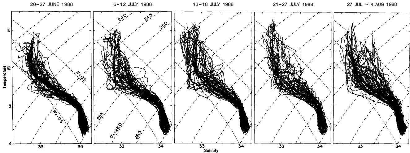
Fig. 13. T - S curves for all stations during each complete survey. Dashed curves sloping up toward the right are lines of constant density anomaly ( \sigma_\theta ), and dashed curves sloping down to the right are lines of constant spiciness ( \pi ).
